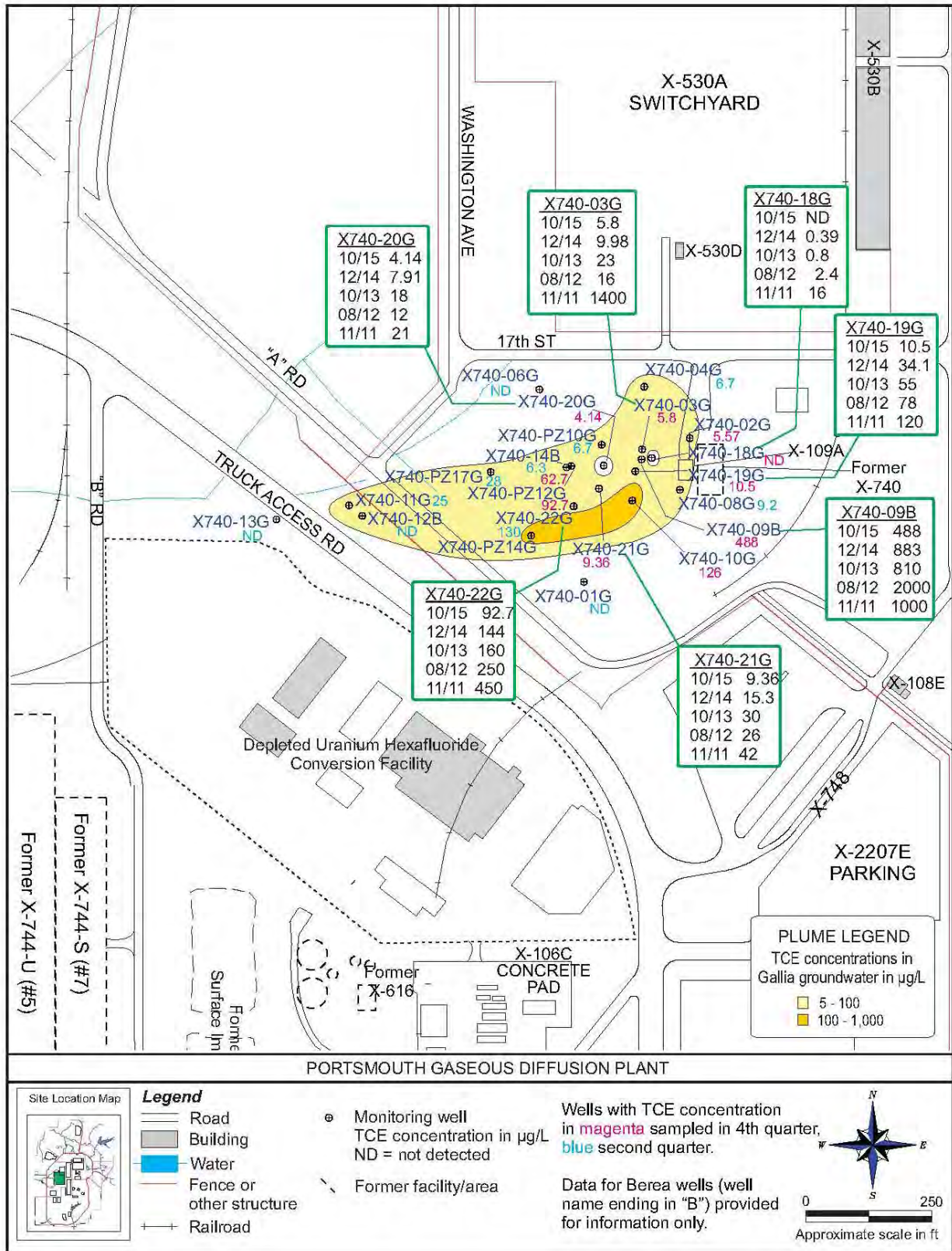
Figure 6.8. TCE-contaminated Gallia groundwater plume near the X-740 Former Waste Oil Handling Facility – 2015.
