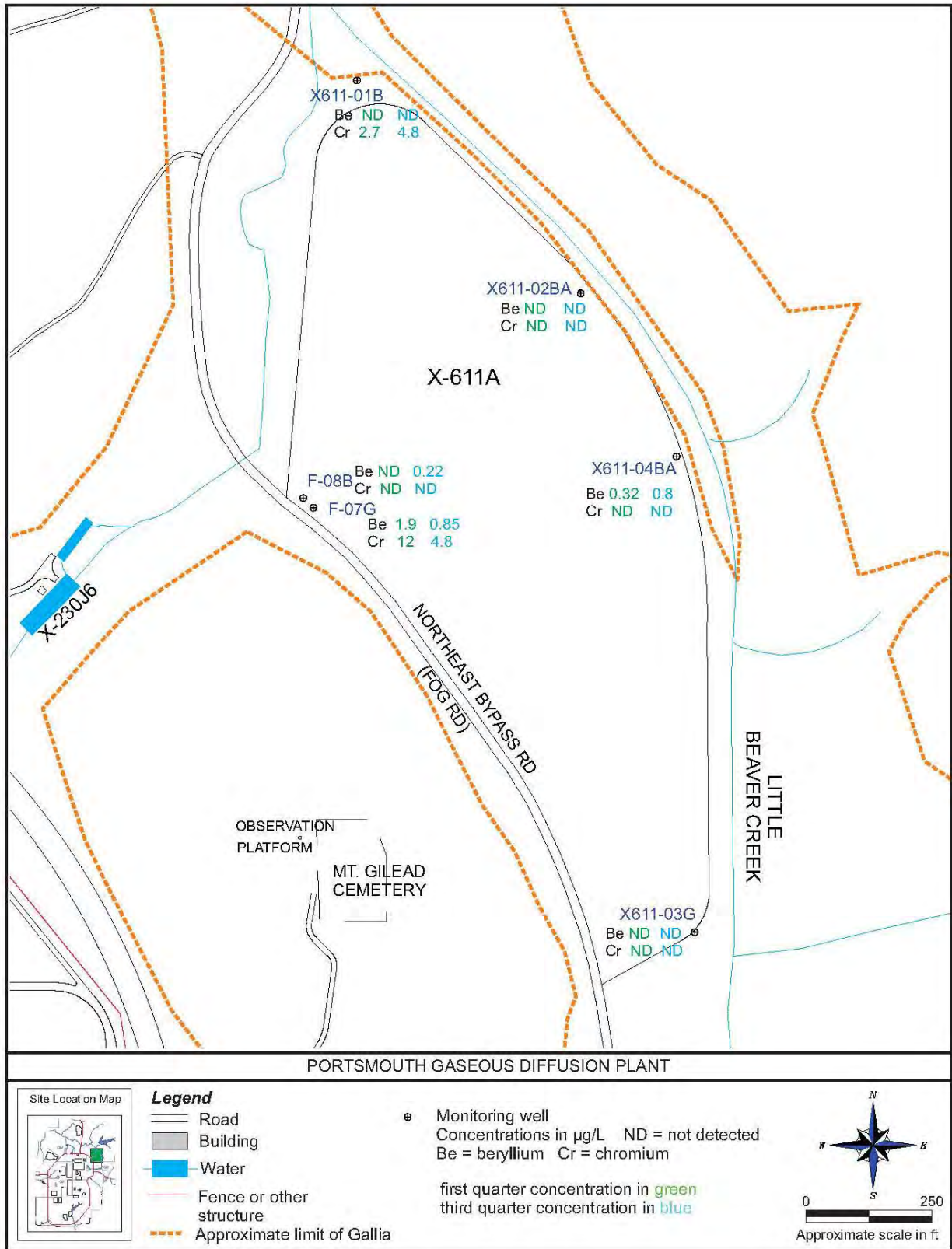
Figure 6.9. Metal concentrations in groundwater at the X-611A Former Lime Sludge Lagoons – 2015.
