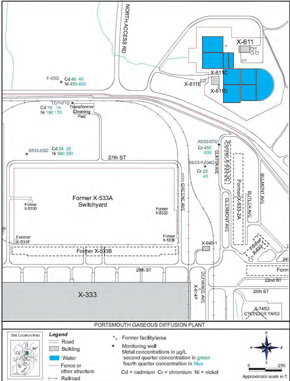
Figure 6.6. Metal concentrations in groundwater at the X-633 Former Recirculating Cooling Water Complex and X-533 Former Switchyard Complex – 2015.
