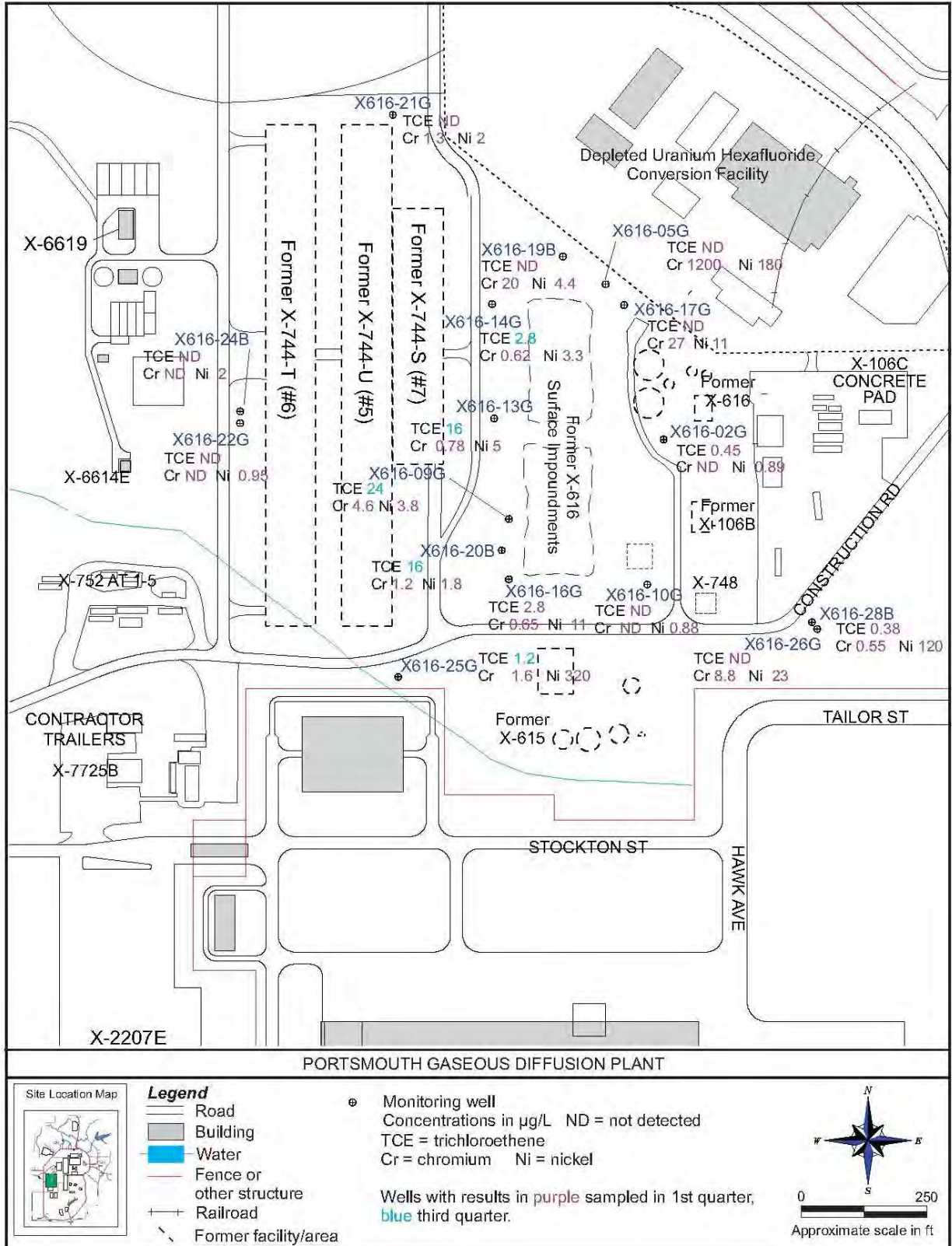
Figure 6.7. TCE and metal concentrations in groundwater at the X-616 Former Chromium Sludge Surface Impoundments – 2015.
